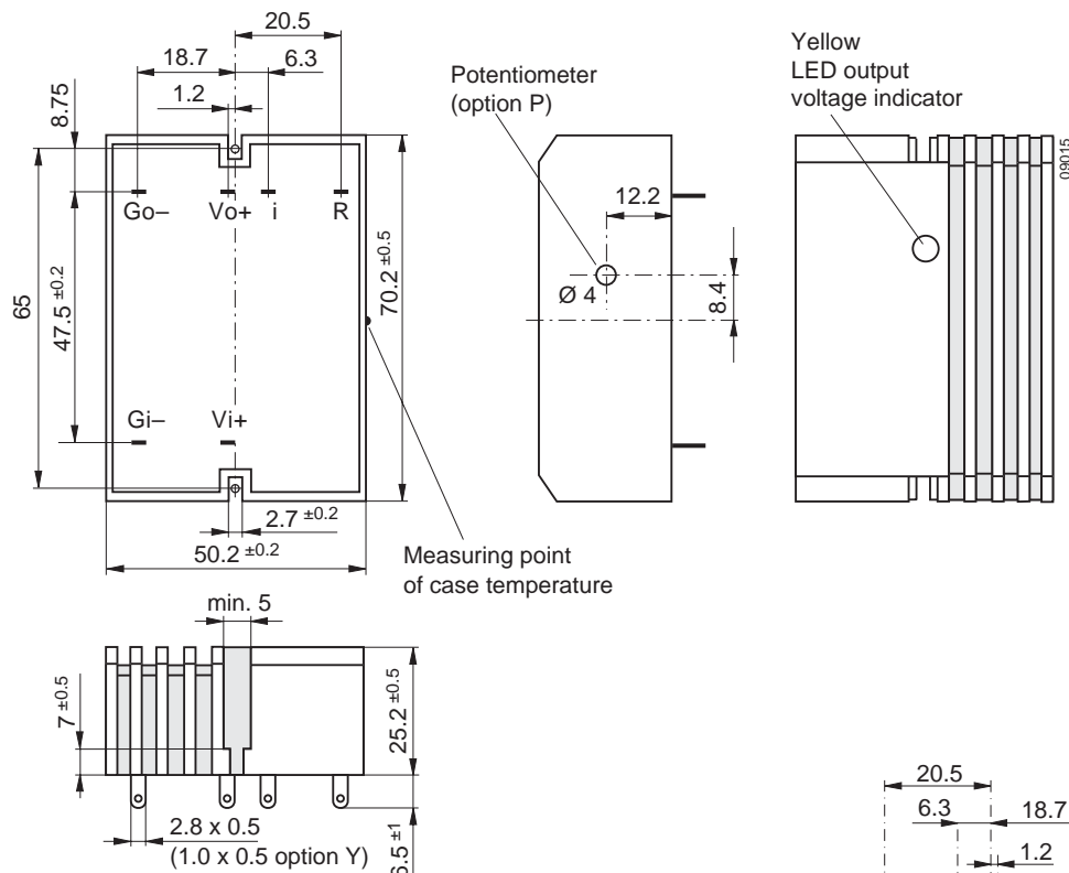
Fig. 7 Case A01, weight 100 g Aluminium, black finish and self cooling
