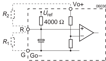
Fig. 13 Voltage adjustment with external resistor R_1 or R_2
