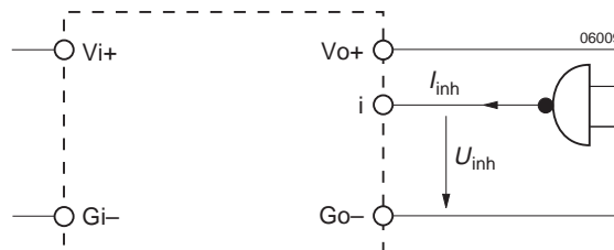
Fig. 10 Definition of I_{inh} and U_{inh}
