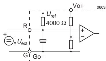
Fig. 12 Voltage adjustment with U_{ext} between R and Go-
