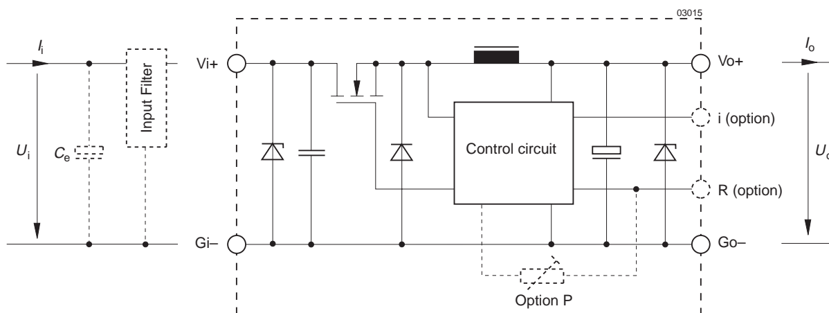
Fig. 1 Block diagram
