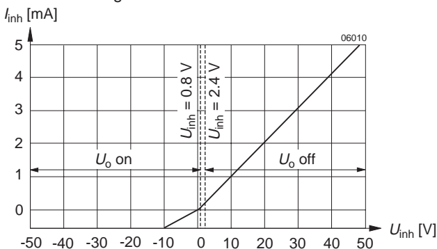
Fig. 9 Typical inhibit current I_{inh} versus inhibit voltage U_{inh}
