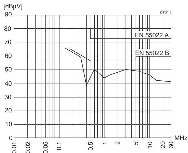
Fig. 6 Typical disturbance voltage (quasi-peak) at the input according to EN 55011/22 measured at U_{i\text{ nom}} and I_{o\text{ nom}} .
