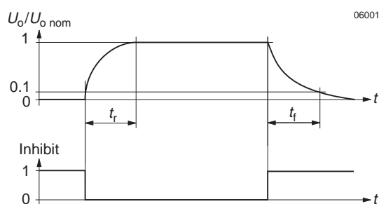
Fig. 11 Output response as a function of inhibit signal
